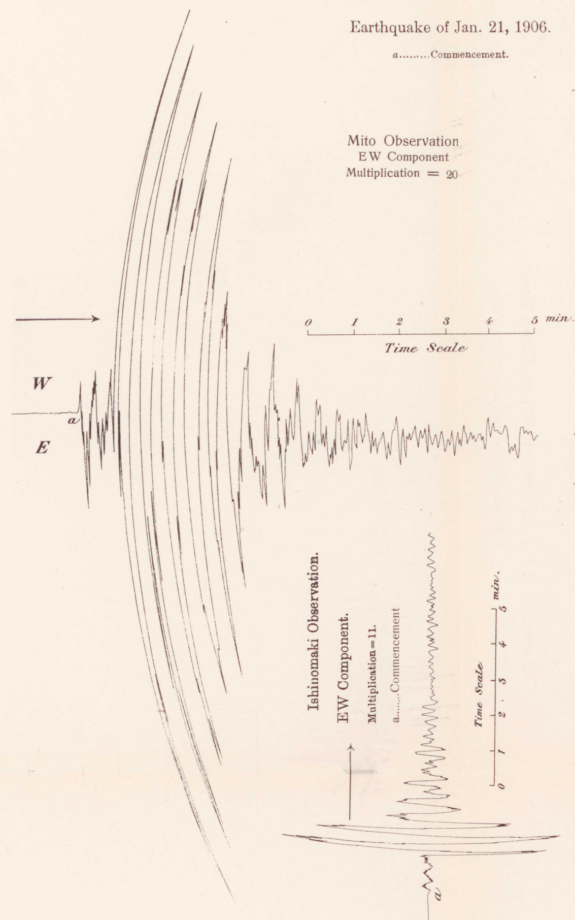
Earthquake of Jan. 21, 1906; 10:50 P.M. (Japan Time).
