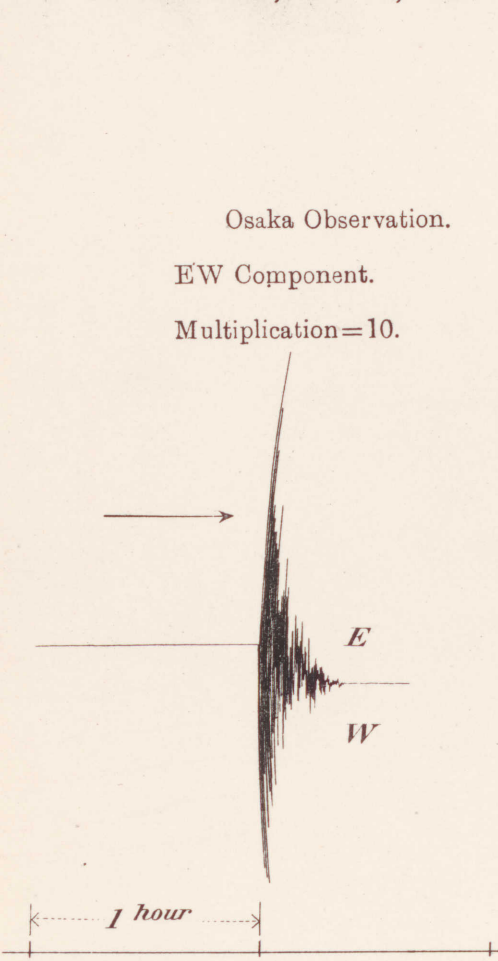
Earthquake of Jan. 21, 1906; 10:50 P.M. (Japan Time).
